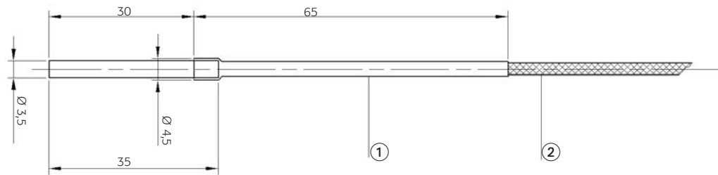
Meßfühler TEF 2 Measuring sensor TEF 2 Thermocouple TEF 2 Sensore di misura TEF 2
