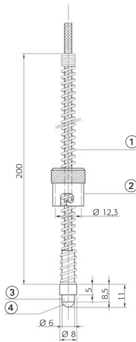
Meßfühler TEF 16B Measuring sensor TEF 16B Thermocouple TEF 16B Sensore di misura TEF 16B
